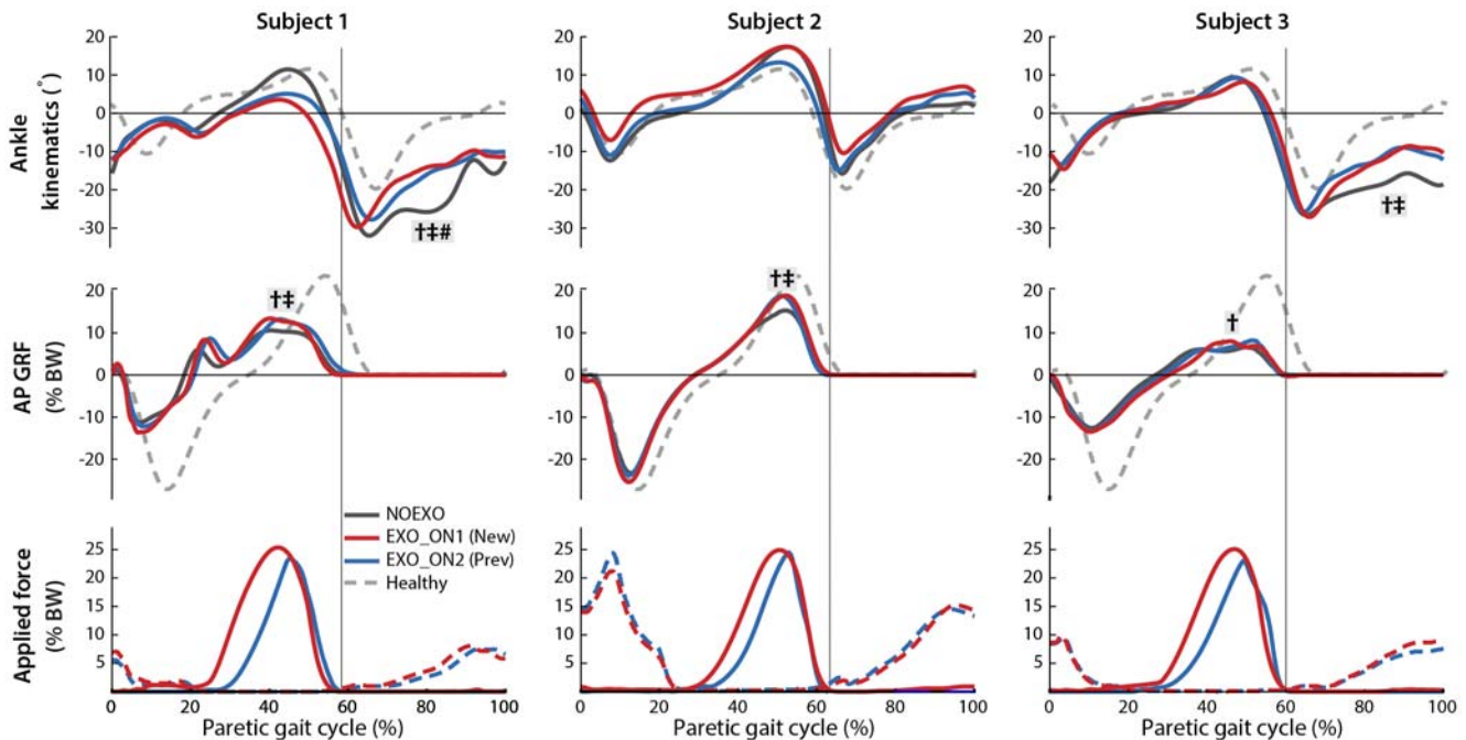
Figure 10. Average biomechanical changes of individual subjects in paretic forward propulsion and ground clearance. (Top) sagittal plane ankle kinematics. (middle) anterior-posterior ground reaction force (AP GRF). (bottom) PF and DF force applied by exosuit. Solid lines are PF forces and dotted lines are DF forces. The vertical lines around 60% GC present paretic toe-off.
